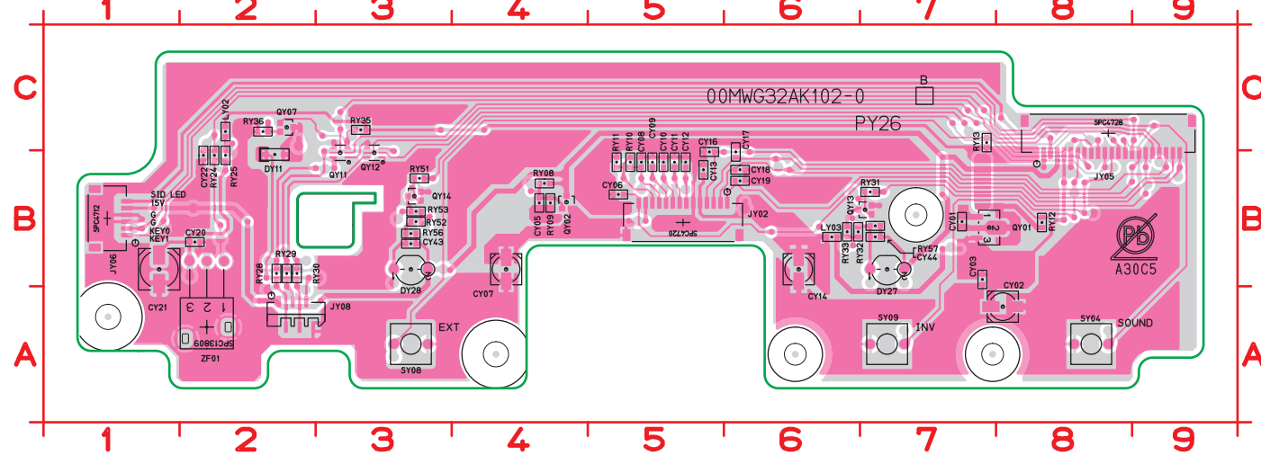
PY26 PWB A
