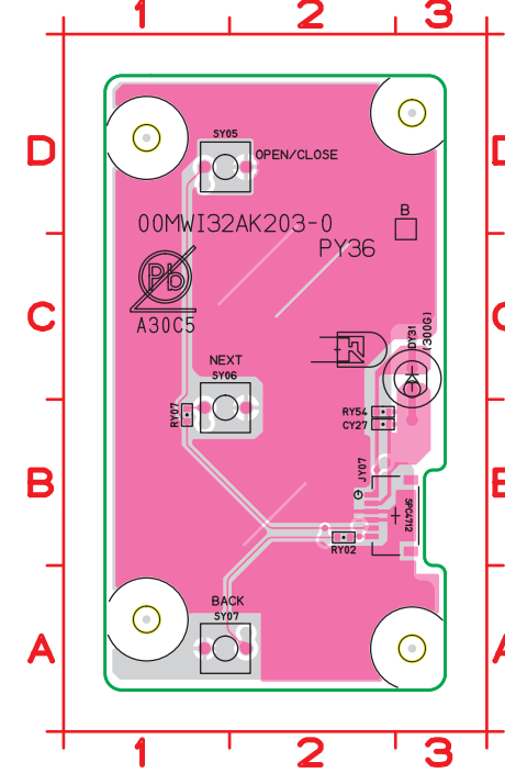
PY36 PWB A
